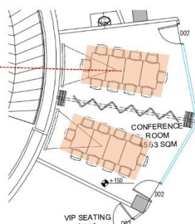
Ceiling plan showing Acoustic grid
