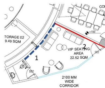
Part plan - VIP Lounge
